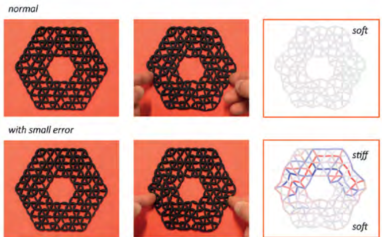
The perfectly composed metamaterial is soft: it completely deforms when you squeeze it. Both experiments and simulations have shown that. However, with a topological error, the structure is different: it becomes soft on one side and hard on the other.
